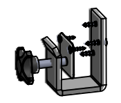
CONNECTOR ASSEMBLY SCALE 1:5
